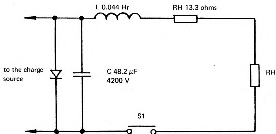
Fig. 3. Simplified diagram of discharge circuit for the 'M' waveform.
